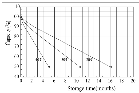
Self-discharge Characteristics
