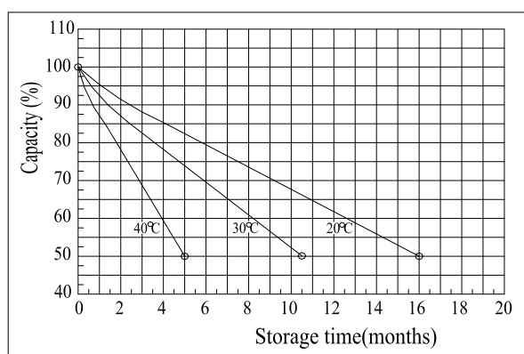
Self-discharge Characteristics
